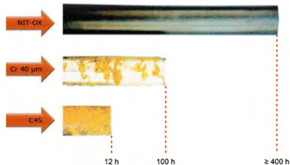
UNI ISO 9227 Salt spray test
